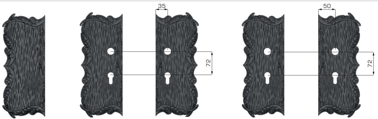
HxL (mm) 310x125 310x125 310x125 310x125 310x125 2 2 2 2 2 new new new new new N° 63.143.00.00 63.144.72.35 63.145.72.35 63.144.72.50 63.145.72.50
